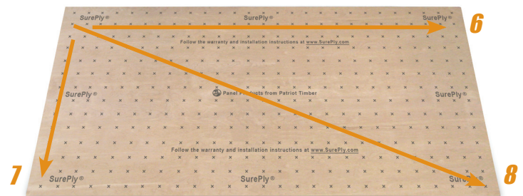
Fastener Diagram 6, 7, 8
